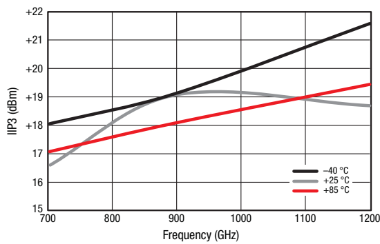
Figure 19. IIP3 vs Frequency Over Temperature
