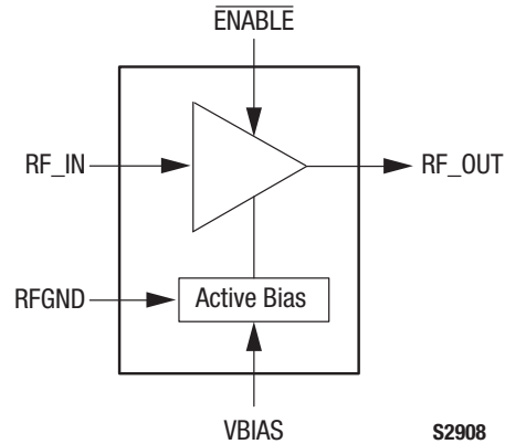
Figure 1. SKY67111-396LF Block Diagram
