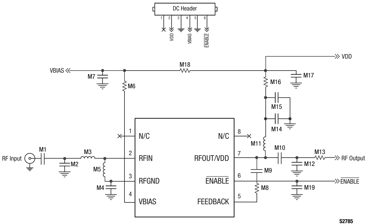
Figure 25. SKY67111-396LF Evaluation Board Schematic
