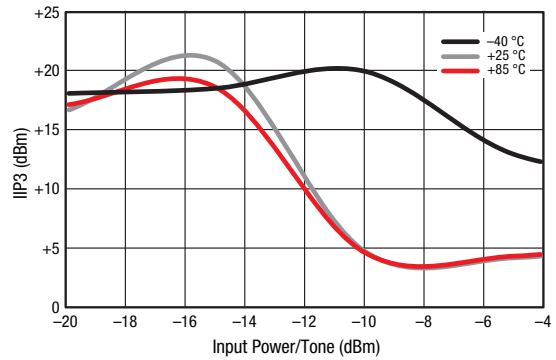
Figure 16. IIP3 vs Temperature (@ 700 MHz)
