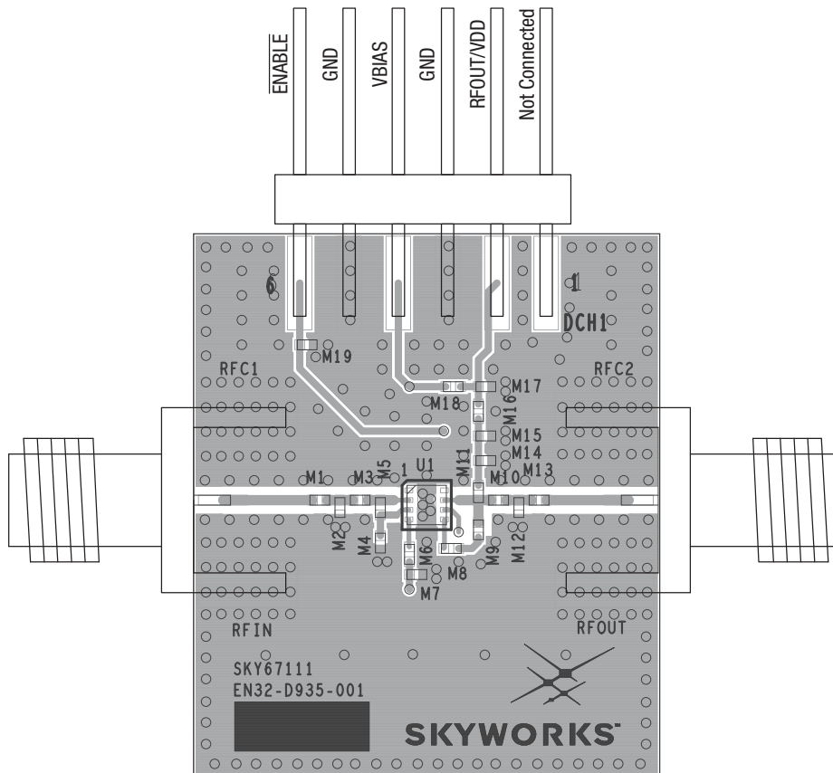
Figure 24. SKY67111-396LF Evaluation Board Assembly Diagram
