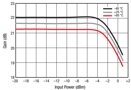
Figure 20. IP1dB vs Temperature (@ 700 MHz)
