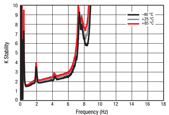
Figure 14. K Stability vs Frequency Over Temperature
