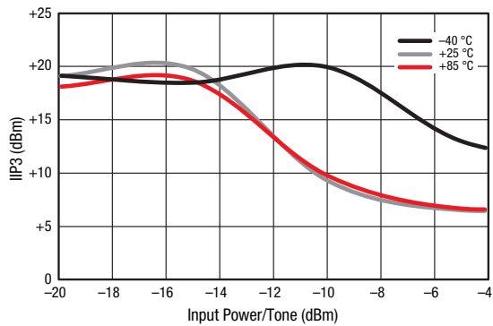
Figure 17. IIP3 vs Temperature (@ 900 MHz)
