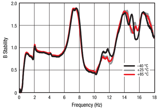
Figure 15. B Stability vs Frequency Over Temperature
