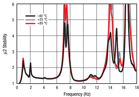
Figure 13. 2 Stability vs Frequency Over Temperature
