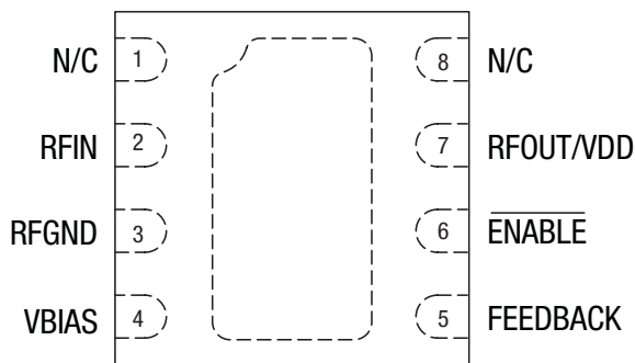
Figure 2. SKY67111-396LF Pinout – 8-Pin DFN (Top View)
