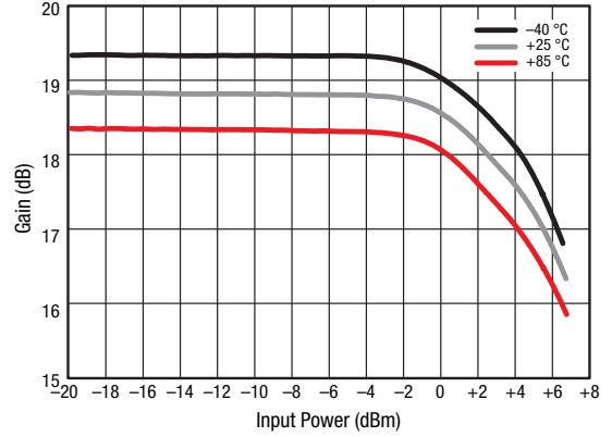
Figure 22. IP1dB vs Temperature (@ 1200 MHz)
