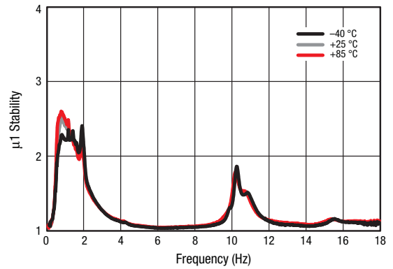
Figure 12. 1 Stability vs Frequency Over Temperature
