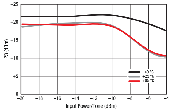
Figure 18. IIP3 vs Temperature (@ 1200 MHz)
